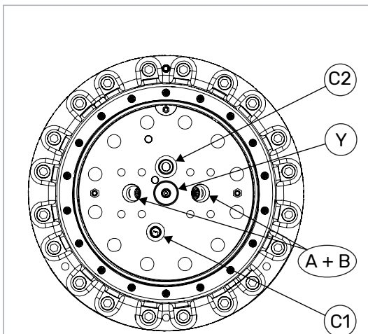
Figure 12. The interface of the motor hydraulics with parking brake.
