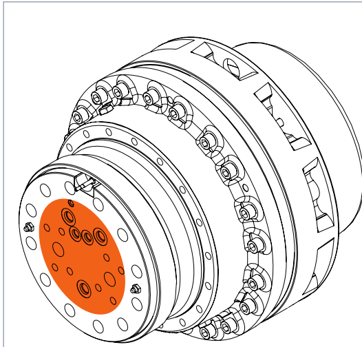
Figure 12. The interface of the motor hydraulics with parking brake.
