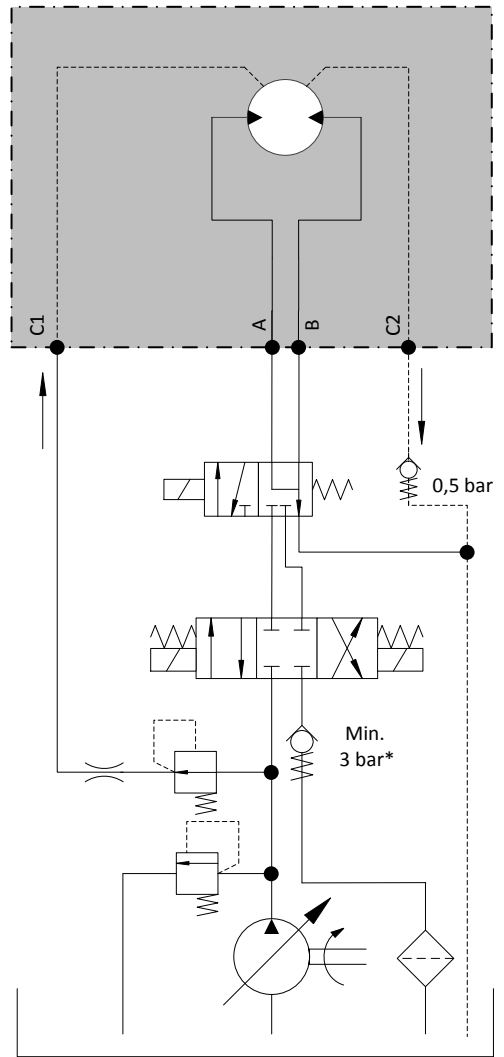
Figure 39. Motor with hydrostatic free-wheeling and external freewheeling valve (open loop).
