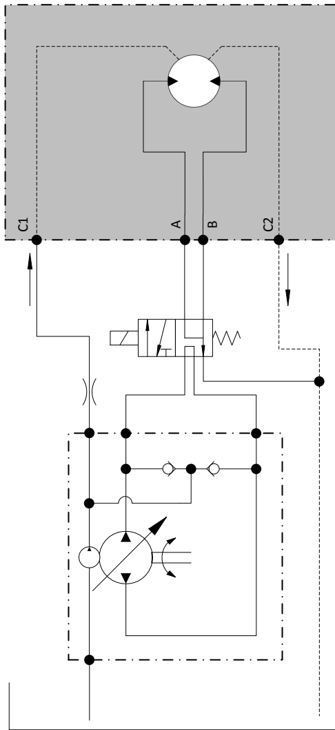
Figure 38. Motor with mechanical free-wheeling and external freewheeling valve (closed loop).
