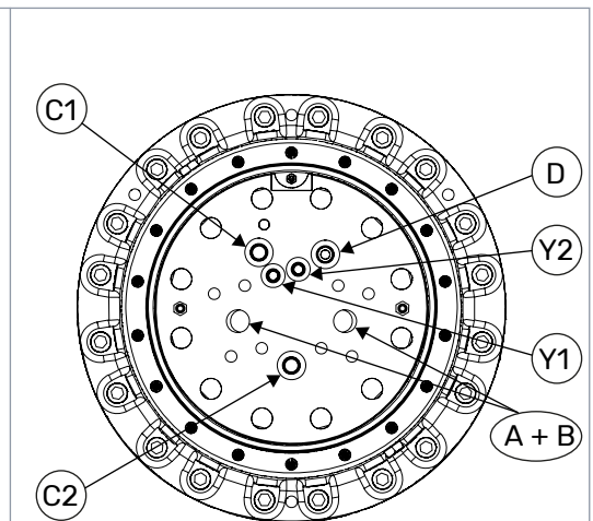
Figure 13. The interface of the motor hydraulics with double brake.
