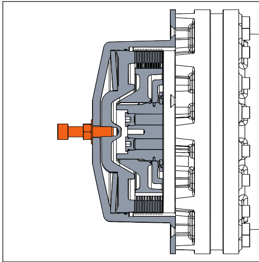
Figure 25. Mechanical brake release
