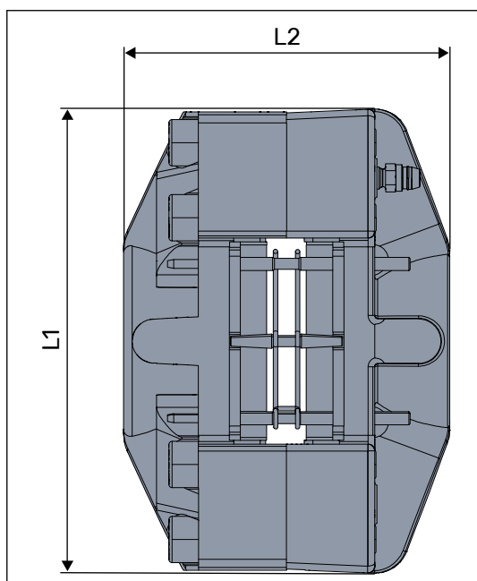
Figure 30. Main dimensions of the brake caliper.
