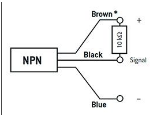
Figure 27. Coupling of the speed sensor.
