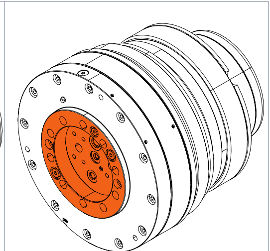
Figure 13. The interface of the motor hydraulics with double brake.
