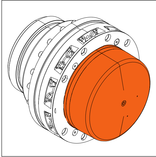
Figure 24. Static wet multi-disc brake
