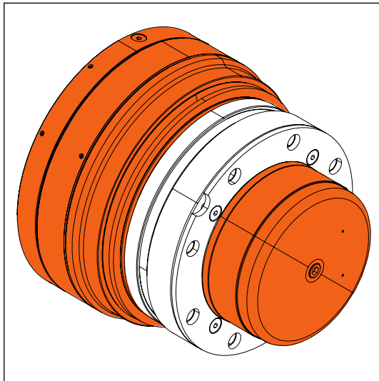
Figure 26. C2x3 motor's double brake
