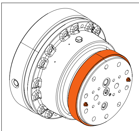
Figure 23. C200 motor's seal protector and grease nipples.
